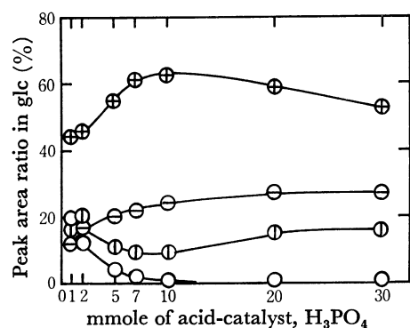
Fig. 1. Effect of supported amount of acid-catalyst, \text{H}_3\text{PO}_4 in the reaction of 1d with formaldehyde. Reaction conditions: Reactants, 1d 10 mmol; (\text{CH}_2\text{O})_n 30 mmol; Solvent, AcOH 10 ml; Reaction temperature, 60 °C; Time, 15 hr.
